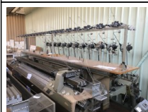
#5: Omatex Straight Weaving Machine
