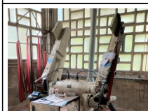
#8: Hau-Samher Double Belt Deburring Machine
